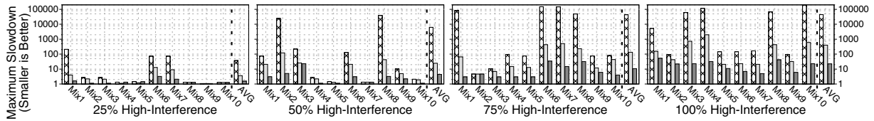
Figure 11: Maximum slowdown of FLIN vs. baseline schedulers.
